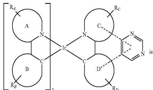
Compound 3
