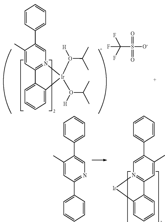
Compound 21
