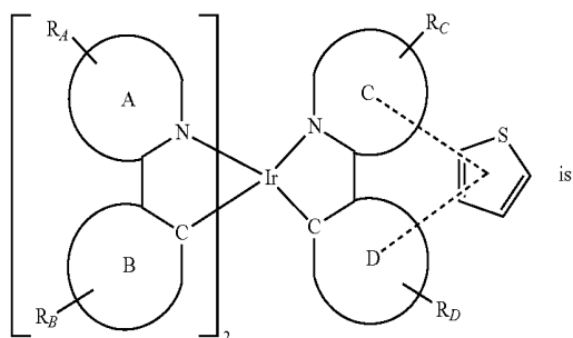
Compound 5
