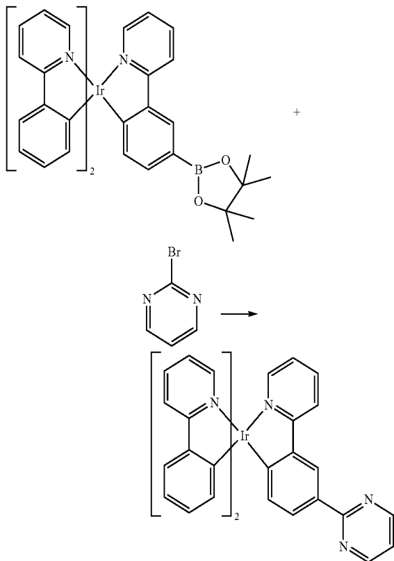
Compound 3
