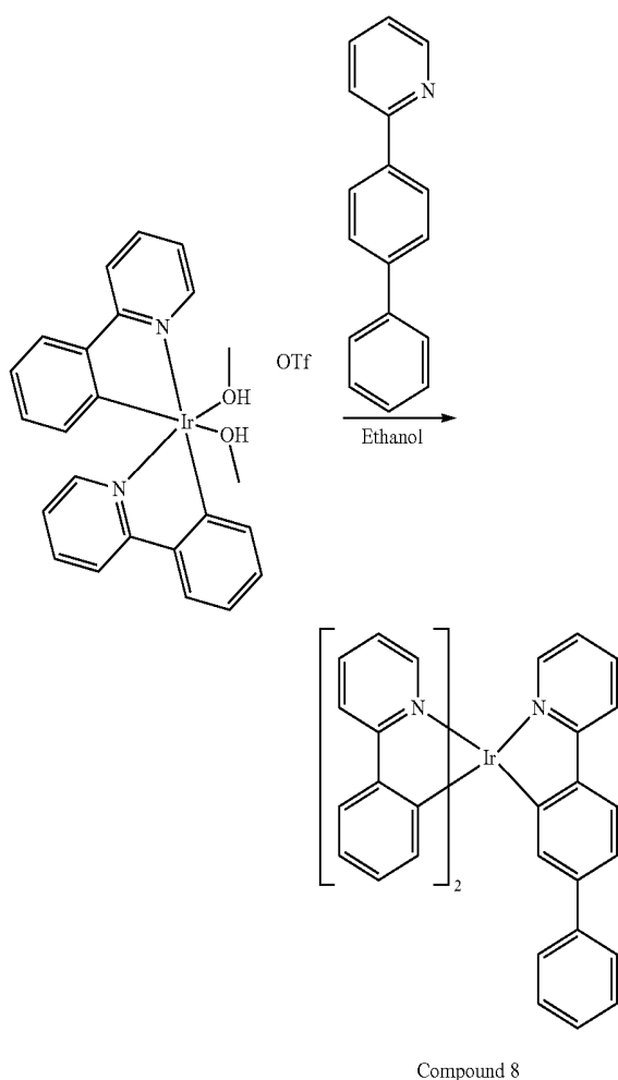
Compound 8
