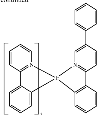
Compound 2
