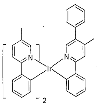
Compound 31
