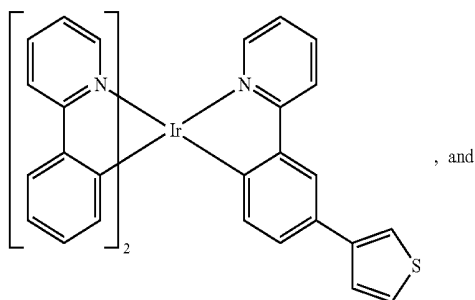
Compound 5
