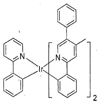
Compound 29
