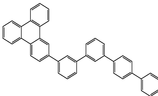
Compound 13
