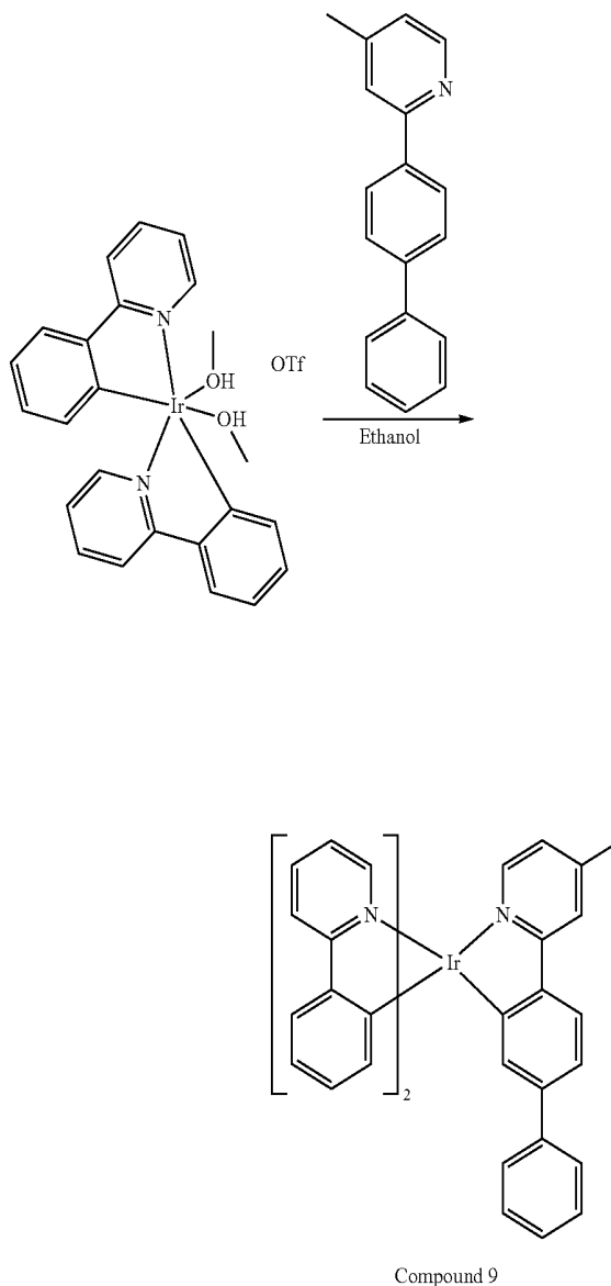
Compound 9
