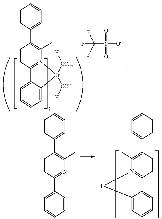
Compound 23
