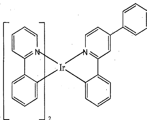
Compound 1
