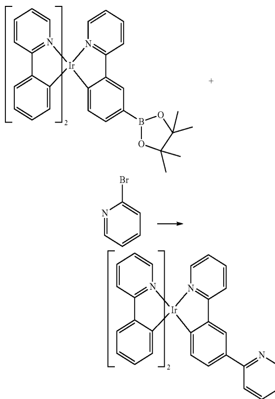
Compound 4
