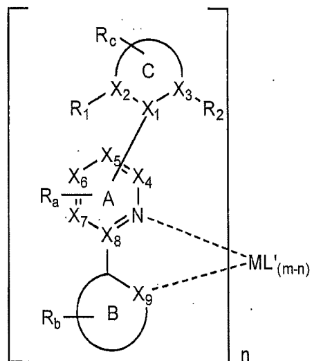
Formula II
