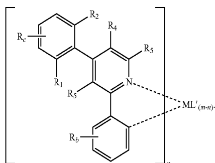
Formula IV
