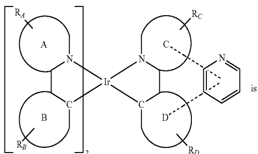
Compound 4
