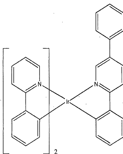
Compound 2
