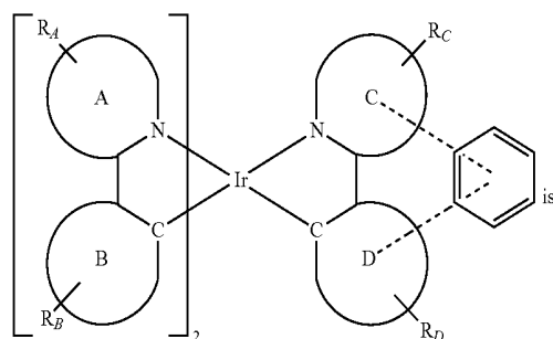
Compound 1
